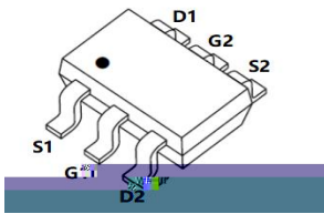
SOT-363-6L Dual top view
